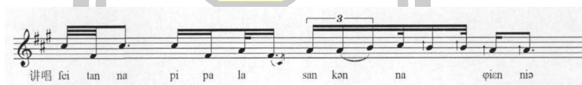
Figure 25 Score : 5-18
